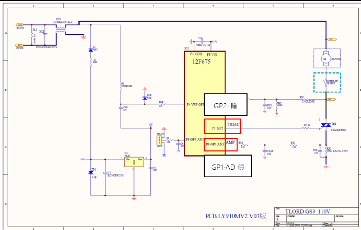
Figure 2: Schematic of Overcurrent
