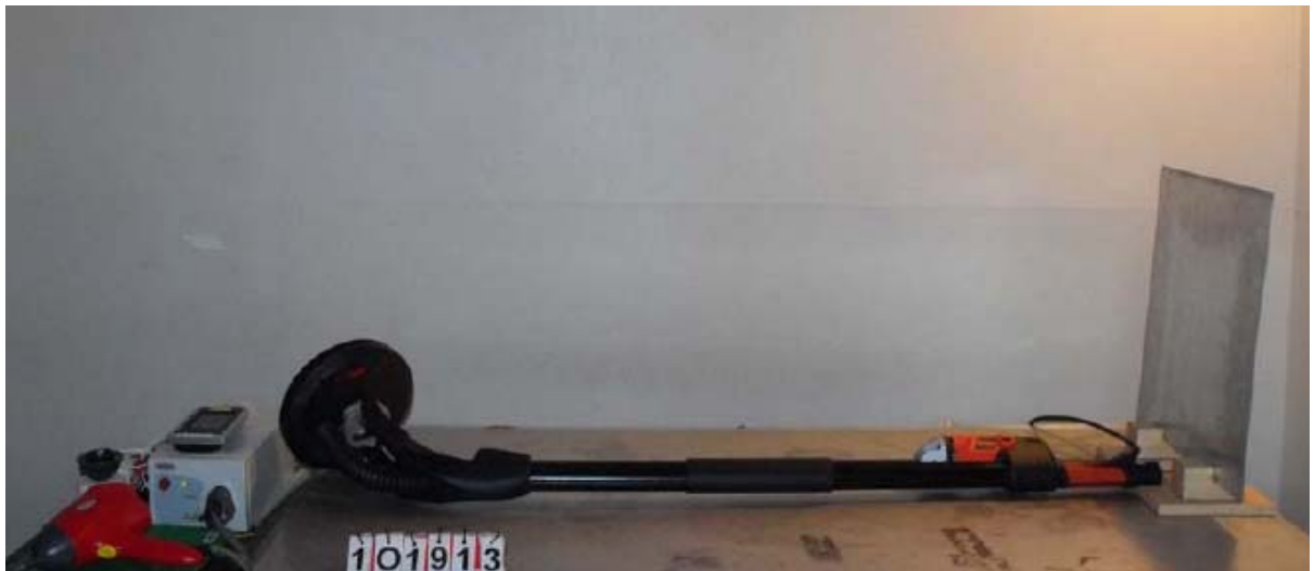
Figure 6 ESD test setup
