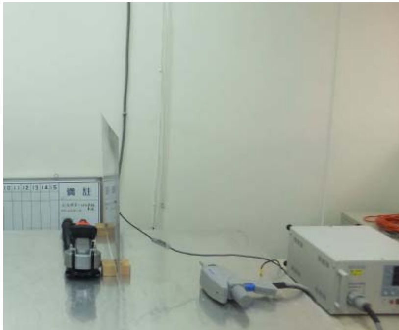
Figure 7 ESD test setup
