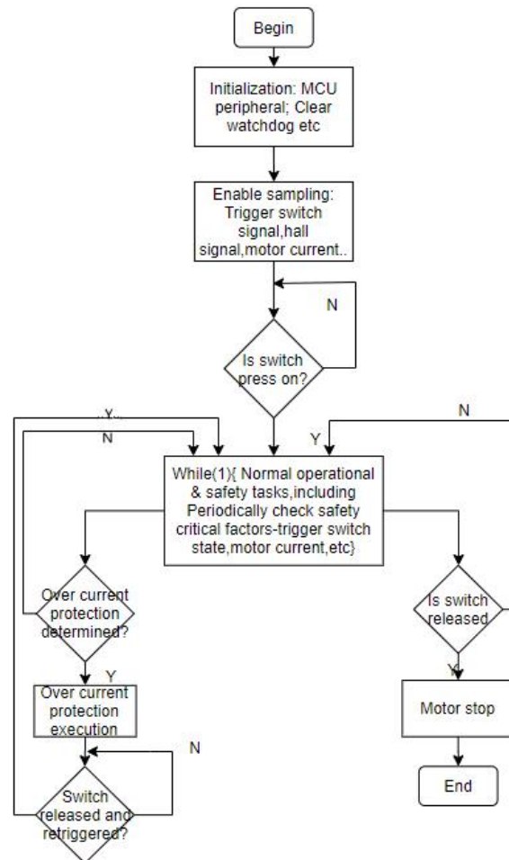
Figure 9: Main Flowchart
