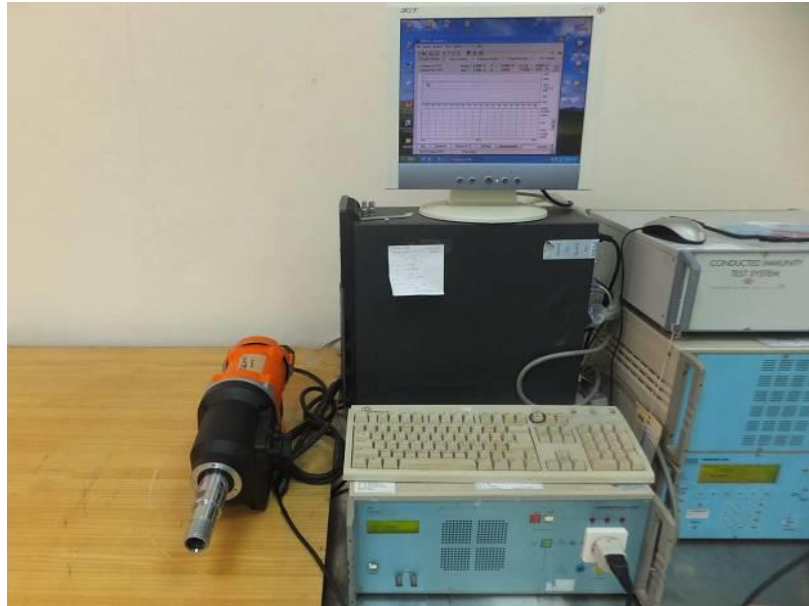
Figure 6 Harmonics & Flicker test setup
