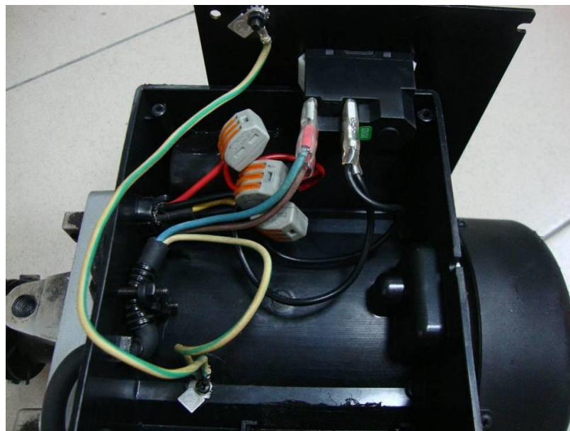
Figure 2 Internal view
